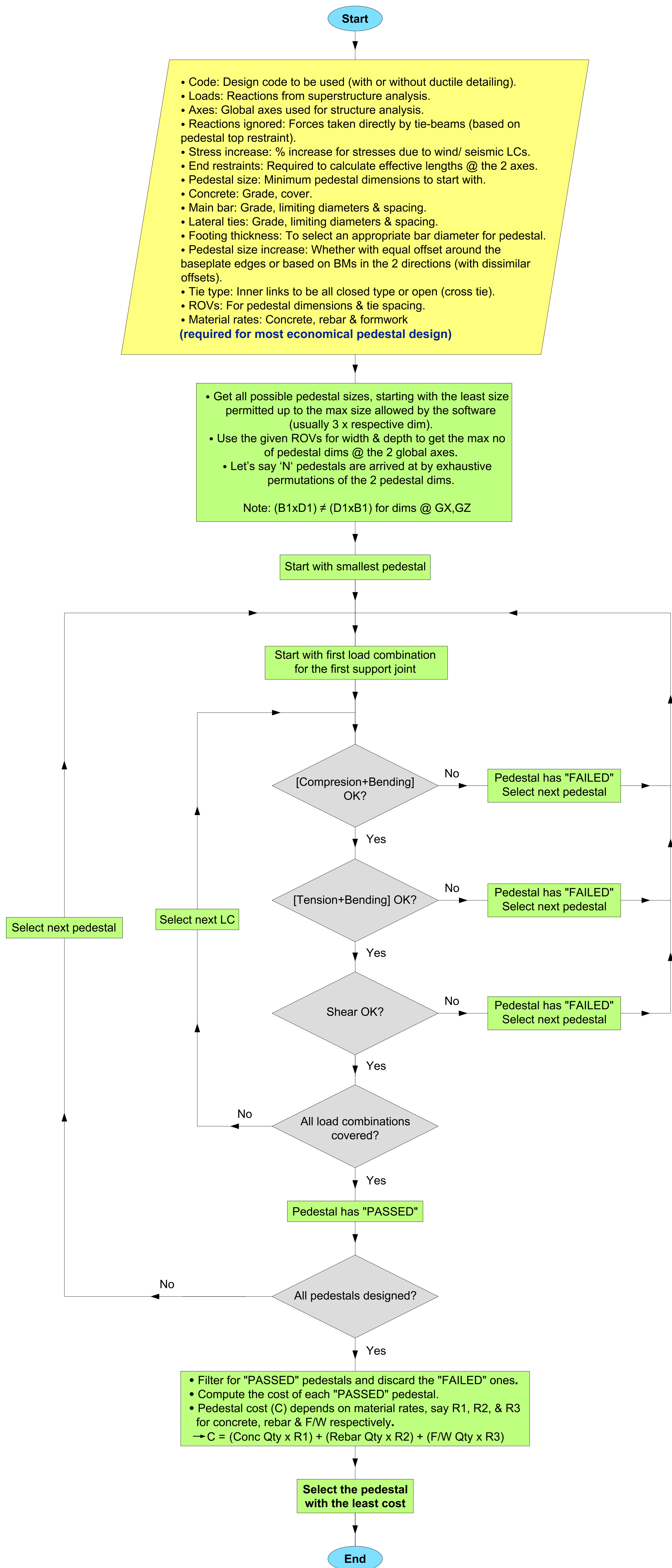
FLOWCHART : MOST ECONOMICAL PEDESTAL DESIGN Conceptualized by Sayed Hyder (Founder Director - StrSof Software Solutions)
